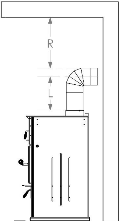
Side view of wall exit Installation
